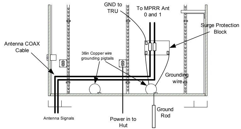
Figure 3 Grounding Diagram
