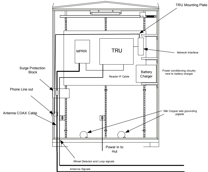
Figure 5 TRU Trackside Hut Interior
