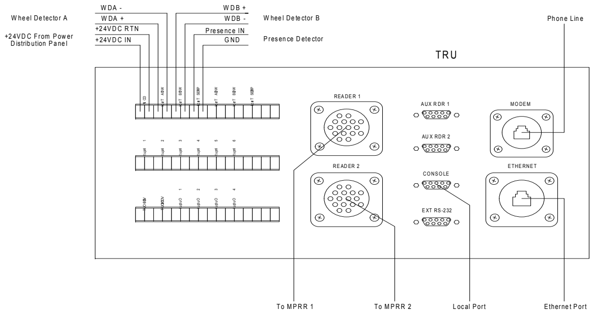
Figure 6 TRU Interface Wiring Diagram
