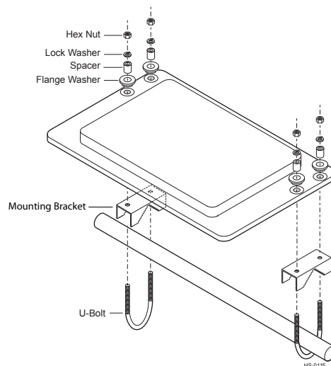
Figure 1 AA3152 Mounting Hardware
